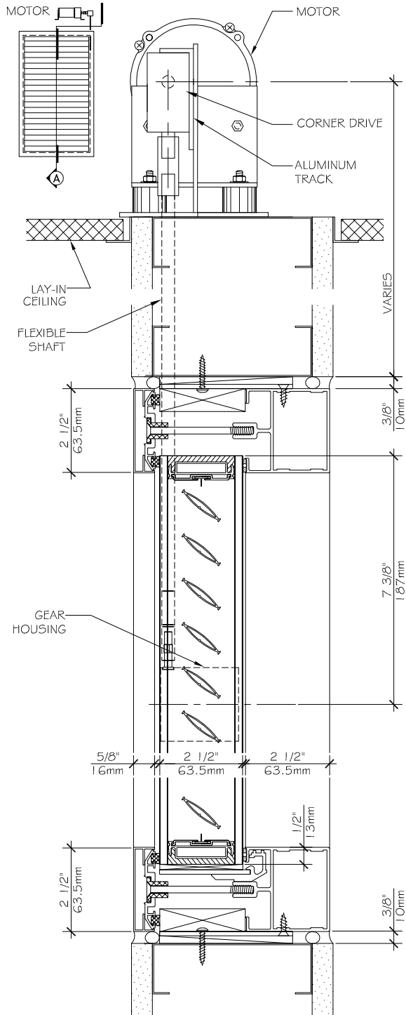
A DETAIL INTERIOR WALL
