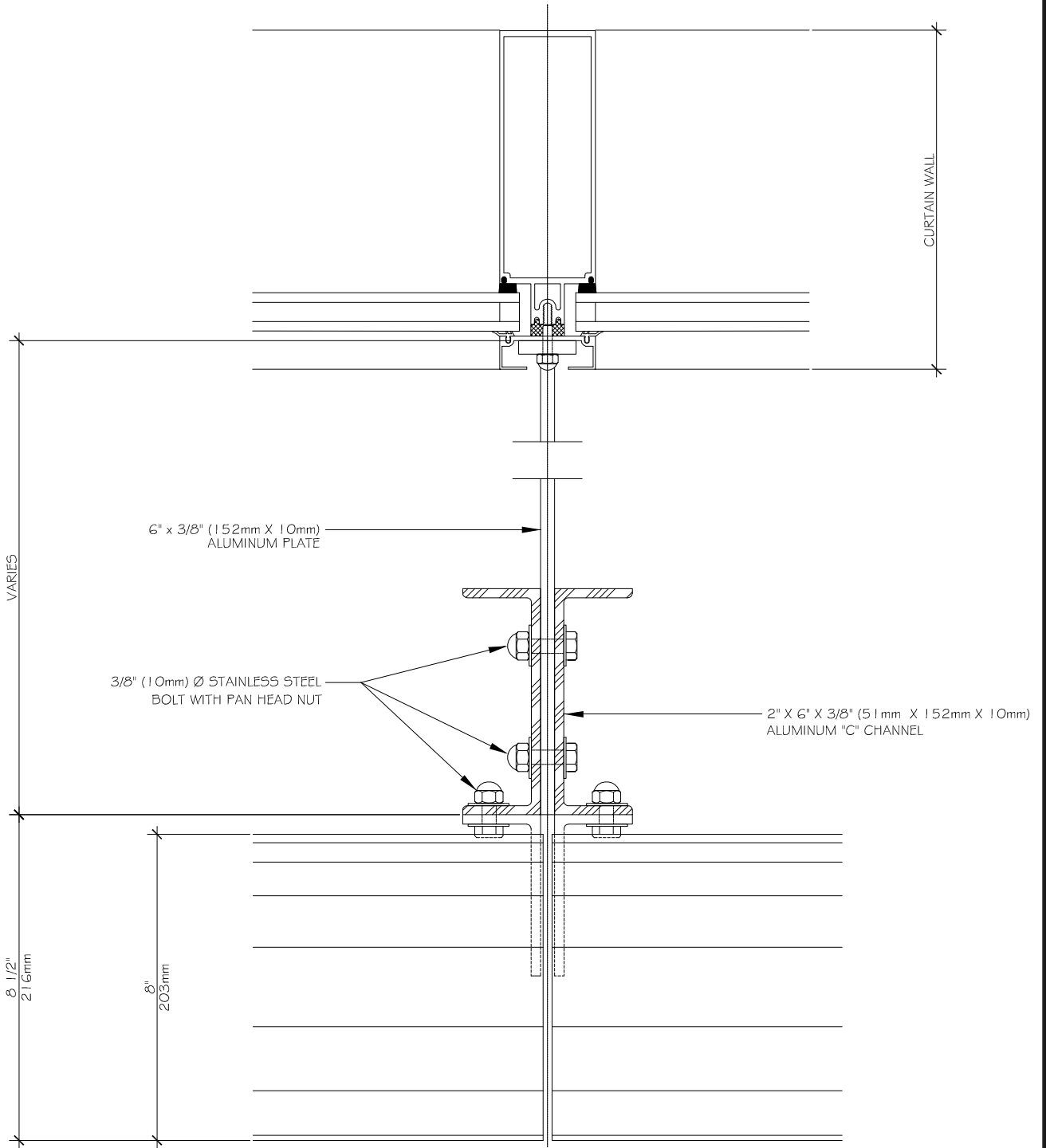
Ⓑ DETAIL (see page cs 3.3)
