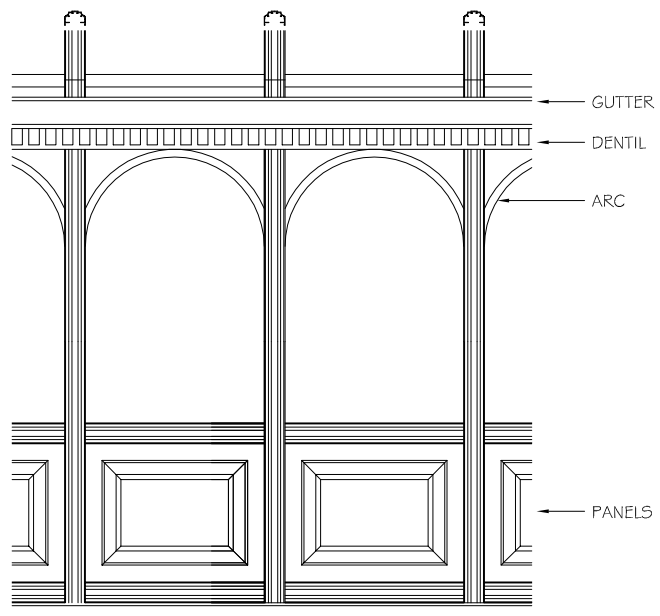
EXTERIOR VIEW
