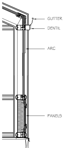
SECTION
