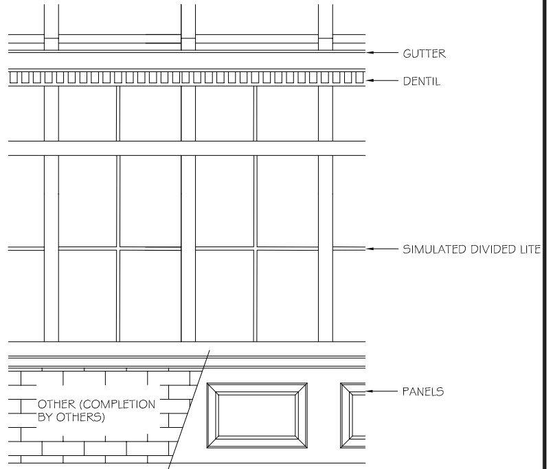
EXTERIOR VIEW
